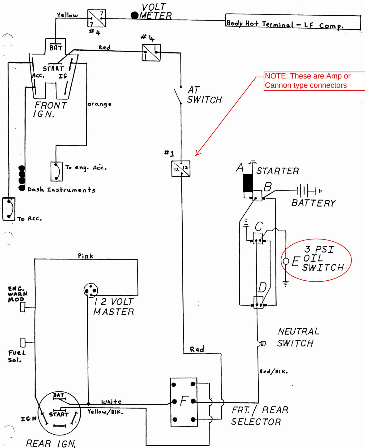
1982 — 1986 PT STARTING CIRCUIT
